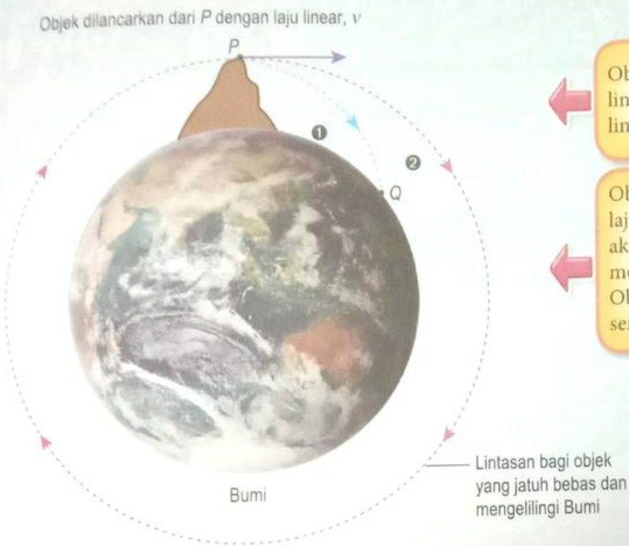
Rajah 3.18 Ramalan Isaac Newton
